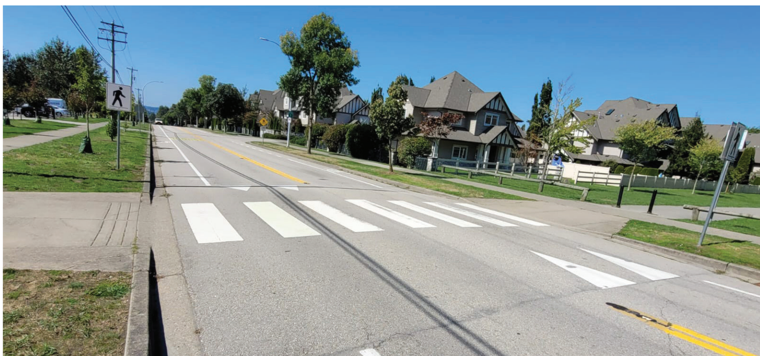
Raised crosswalk
